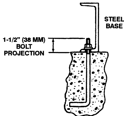
Figure 1. Anchor Hardware Installation
