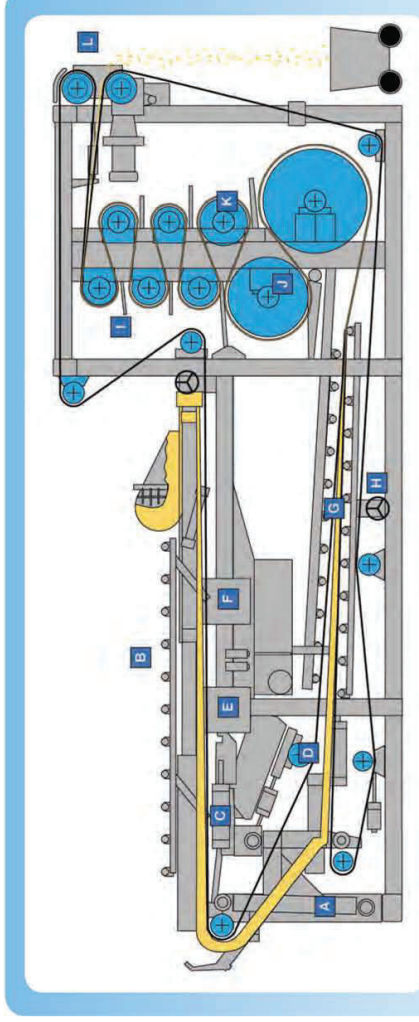
The Model TP7.4 Tower™ Press uses a drum instead of a gravity deck to minimize its footprint. This provides smaller plants with the same high performance dewatering results as larger presses, but for almost half the cost.
